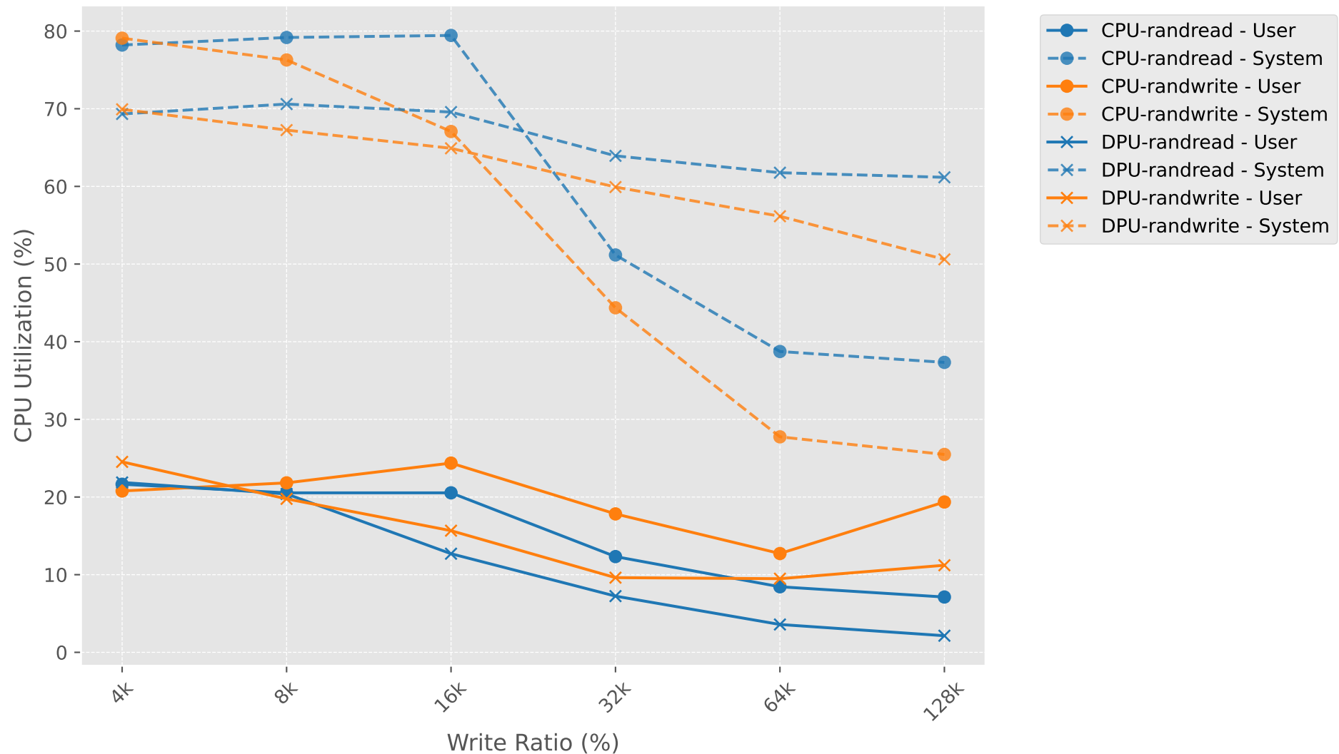
CPU Utilization vs Write Ratio (bs)
